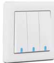
3G Switch Illuminated BR010701 20 A - 16 AX, 250 V~ BS EN 60669-1
