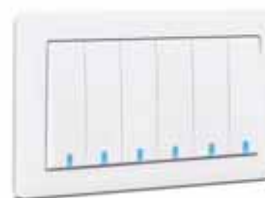
6G Switch Illuminated BR015401 20 A - 16 AX, 250 V~ BS EN 60669-1
