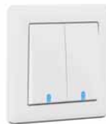
2G Switch Illuminated BR010601 20 A - 16 AX, 250 V~ BS EN 60669-1
