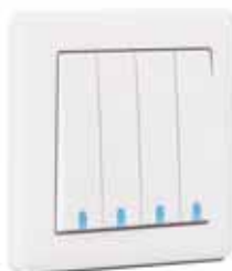
4G Change-Over Switch Illuminated BR011601 20 A - 16 AX, 250 V~ BS EN 60669-1
